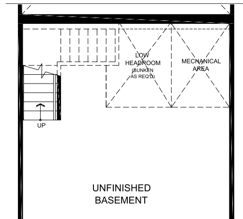
ELEVATION B1 PARTIAL BASEMENT W/O SUNKEN AREA
