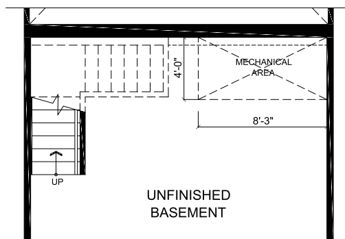
ELEVATION A1 PARTIAL BASEMENT W/O SUNKEN AREA
